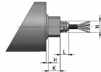
Straight connector.
